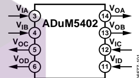
Figure 3. ADuM5402
