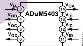
Figure 4. ADuM5403
